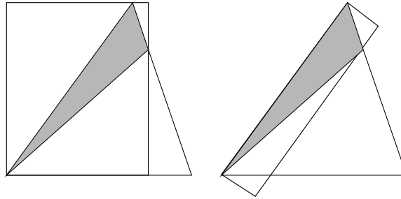
Fig. 4. For non-axis-aligned sliver cut elements (shaded area), the original bounding box (left) is rotated to obtain a tighter fit (right). Also shown is the original triangle from which the sliver element was cut.
