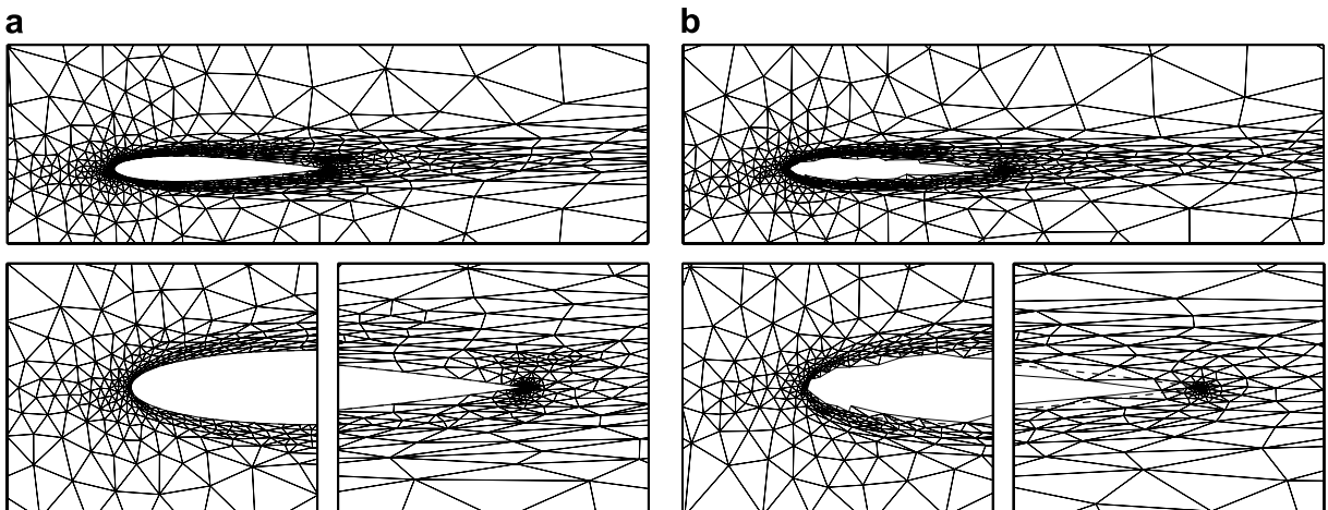
Fig. 9. (a) Boundary-conforming: 1929 elements and (b) cut cell: 1840 elements. Final p = 3 meshes adapted on drag.
