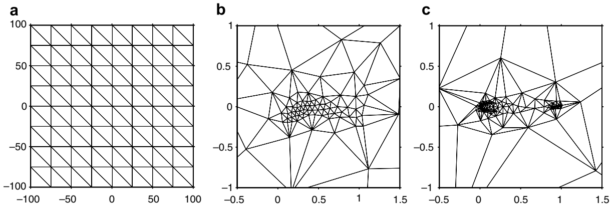
Fig. 10. (a) Uniform 8 \times 8 , (b) adapted on geometry: 245 elements, (c) adapted on geometry: 478 elements. Initial meshes for sensitivity study.
