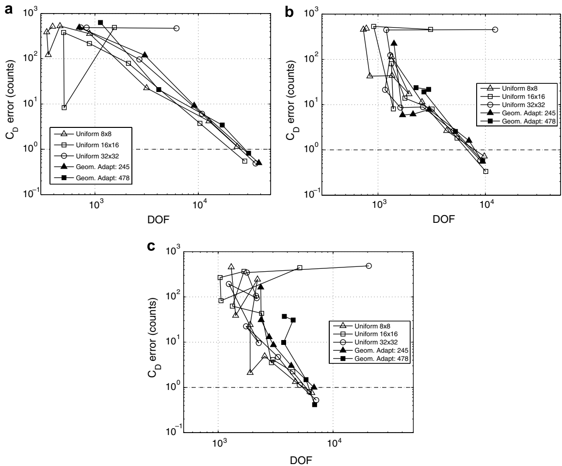
Fig. 11. (a) p = 1 , (b) p = 2 , (c) p = 3 . Adaptation histories starting from the various initial meshes shown in Fig. 10.
