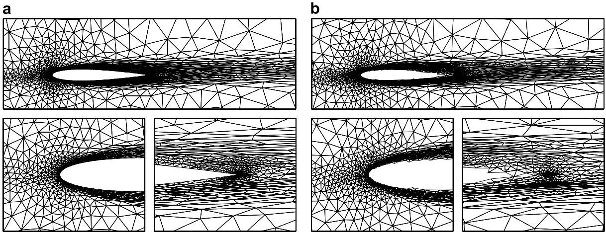
Fig. 8. (a) Boundary-conforming: 3852 elements and (b) cut cell: 4399 elements. Final p = 2 meshes adapted on drag.
