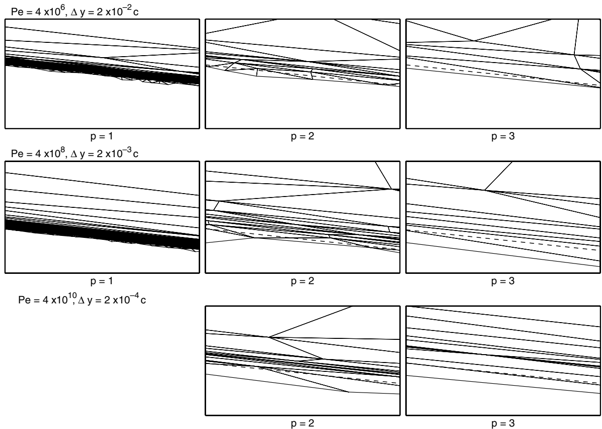
Fig. 13. Close-ups of the boundary-layer meshes for each of the runs. Dashed line indicates the airfoil boundary. \Delta y refers to the y -axis range in each of the plots, in terms of the airfoil chord length, c .
