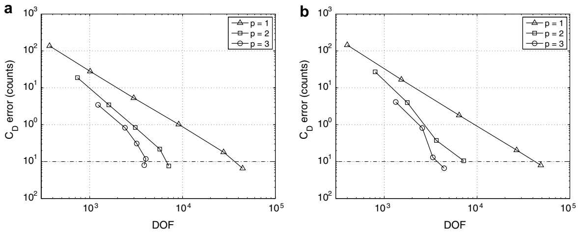
Fig. 6. (a) Boundary-conforming and (b) cut-cell drag error vs. degrees of freedom for the inviscid NACA 0012 runs.
