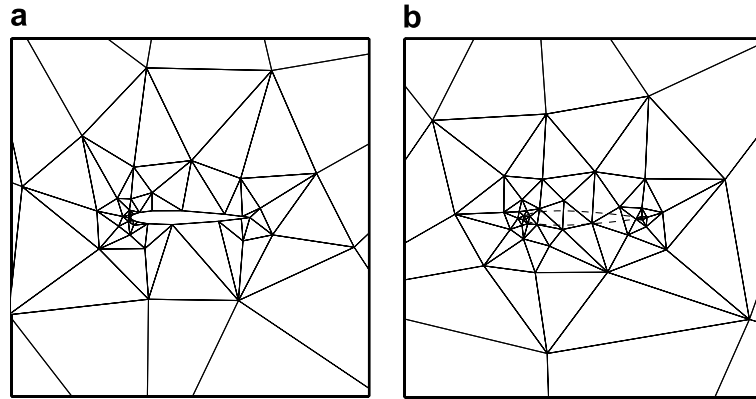
Fig. 5. (a) Boundary-conforming: 123 elements, (b) cut cell: 124 elements initial NACA 0012 meshes.
