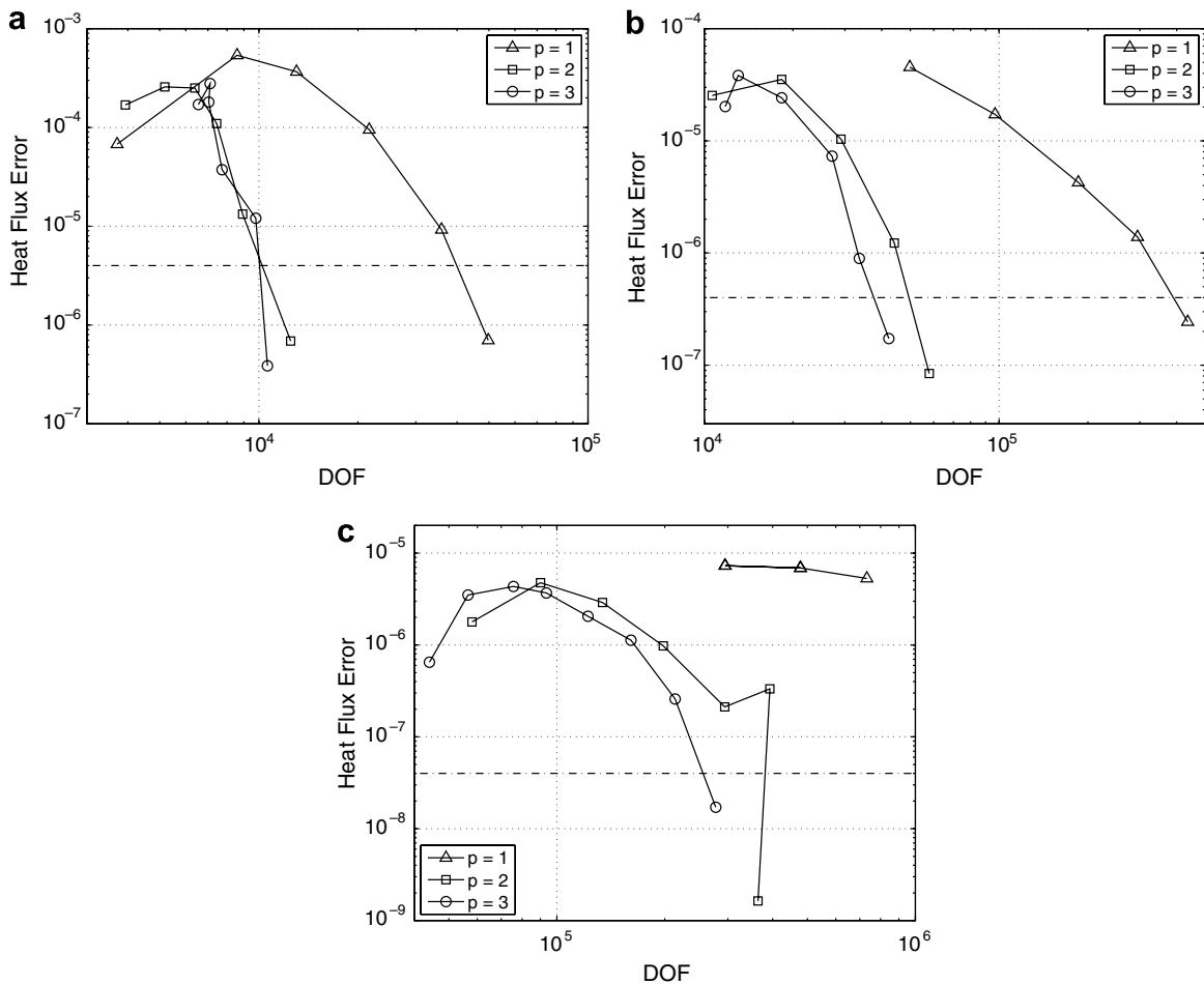
Fig. 12. (a) Pe = 4 \times 10^6 , (b) Pe = 4 \times 10^8 and (c) Pe = 4 \times 10^{10} . Output error vs. DOF adaptation history.
