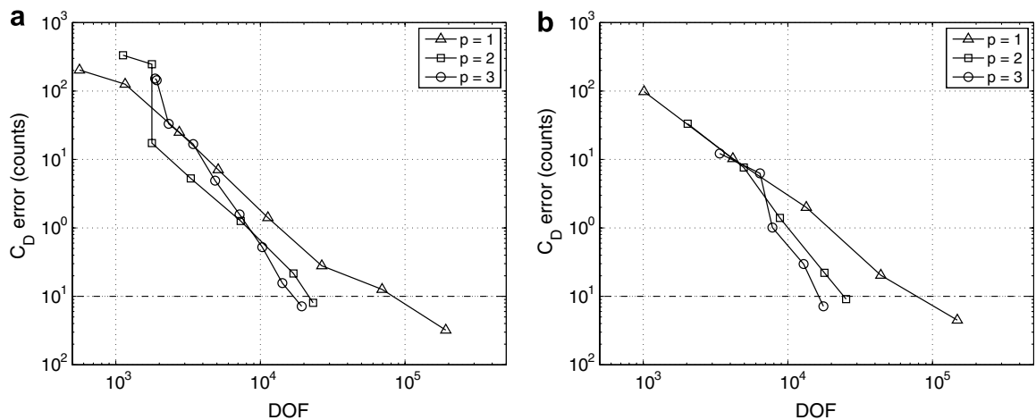
Fig. 7. (a) Boundary-conforming and (b) cut-cell drag error vs. degrees of freedom for the viscous NACA 0012 runs. The dashed line indicates prescribed tolerance of 0.1 drag counts.
