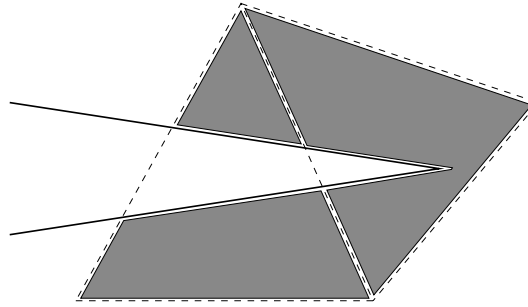
Fig. 1. Shaded areas illustrate cut cells formed at an airfoil trailing edge.
