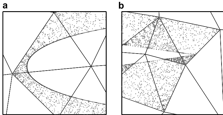
Fig. 3. (a) Leading edge and (b) trailing edge example of sampling points on a cut NACA 0012 mesh.
